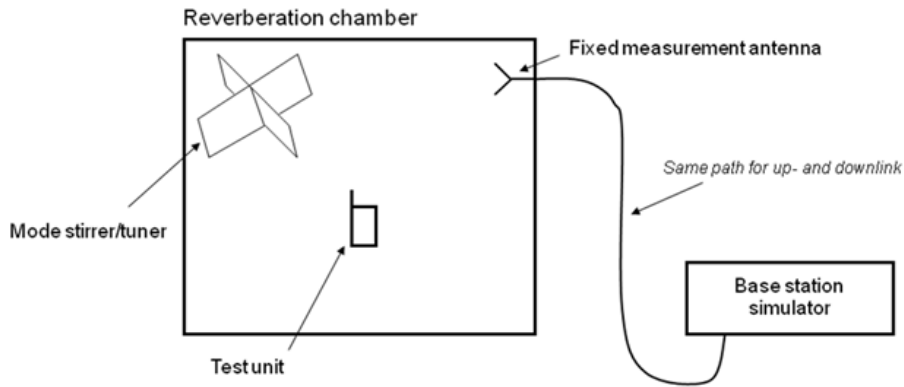
Figure 4.2.1.1-1 Reverberation chamber measurement setup
