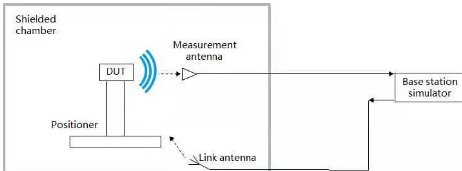
Figure 4.1.1-1: Simplified block diagram showing for a common configuration for the use of a base station simulator for TRP measurements
