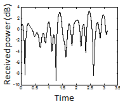
Figure 4.2.1-2 Rayleigh faded signal in reverberation chamber
