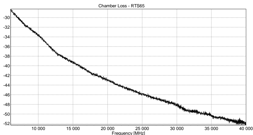
Figure 4.2.1-1 Chamber loss
