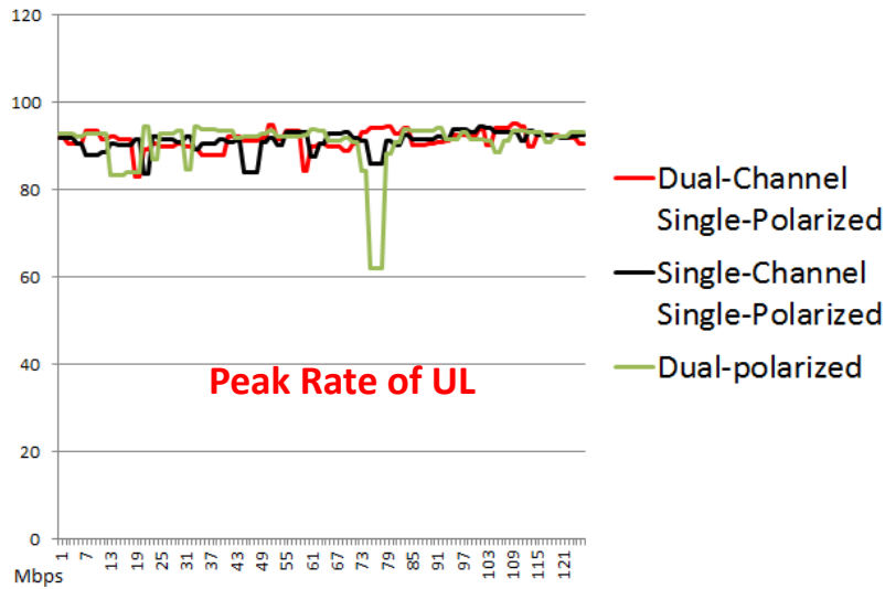
Figure 7-22 DAS Indoor Test Results
