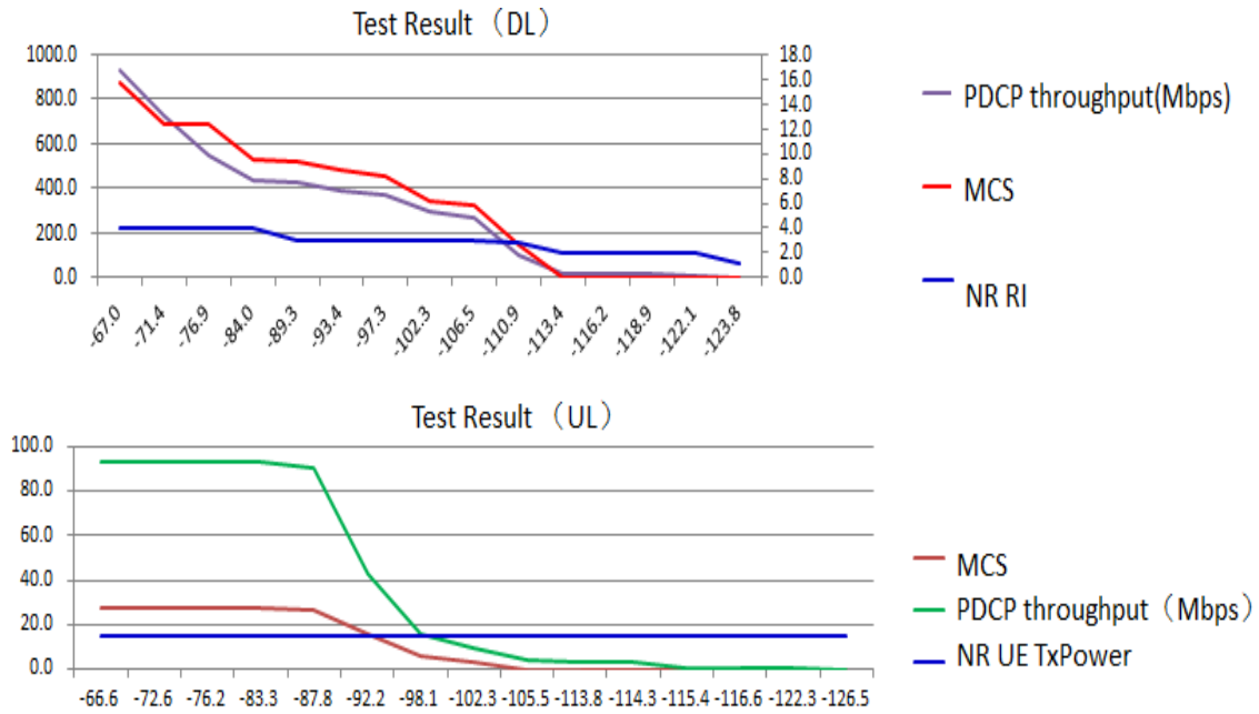
Figure 7-21 DL & UL Test Results in NSA with TDD LTE Anchor
