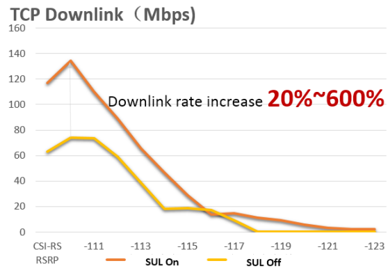
Figure 7-4 Coverage test with SUL On/Off
