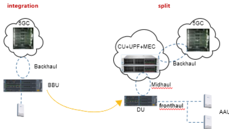
Figure 7-20 Network Deployment and Architecture
