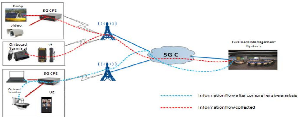
Figure 7-23 Smart navigation network scheme
