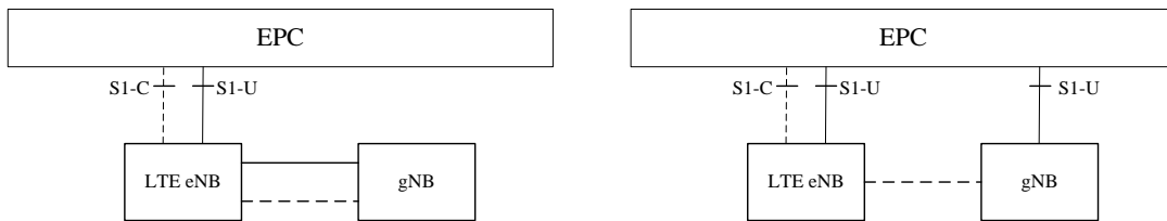
Figure 8-2 Non-Standalone NR – 3GPP Option 3 and 3A
