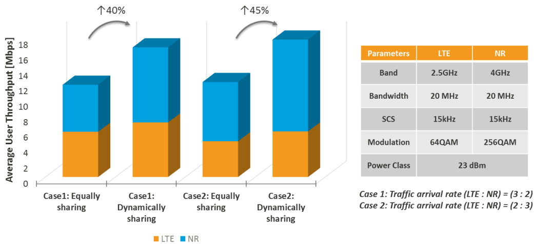
Figure 11-9 EPS vs. DPS, Average User Throughput Comparison
