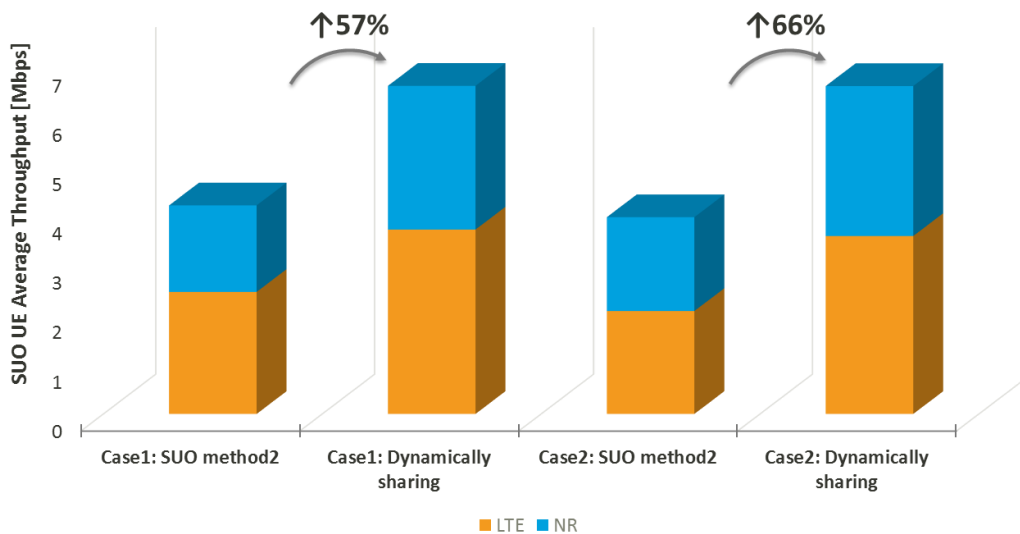
Figure 11-11 Average User Throughput of SUO UE
