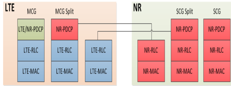
Figure 8-8 NR PDCP aggregation/split for MCG and SCG radio bearer split support in NSA Option3/3x
