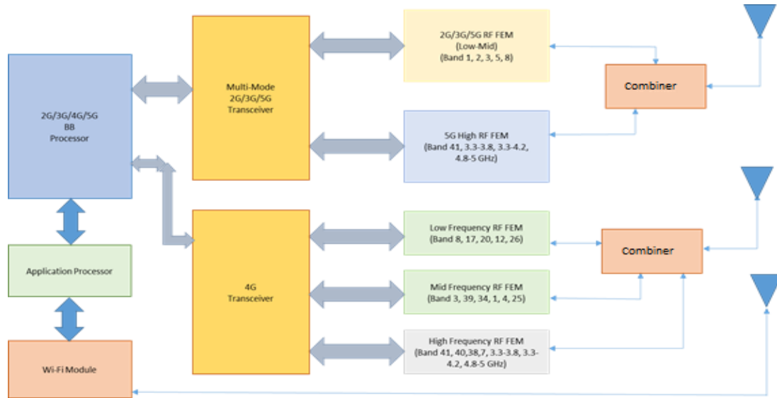
Figure 7-2 MMMB architecture 2
