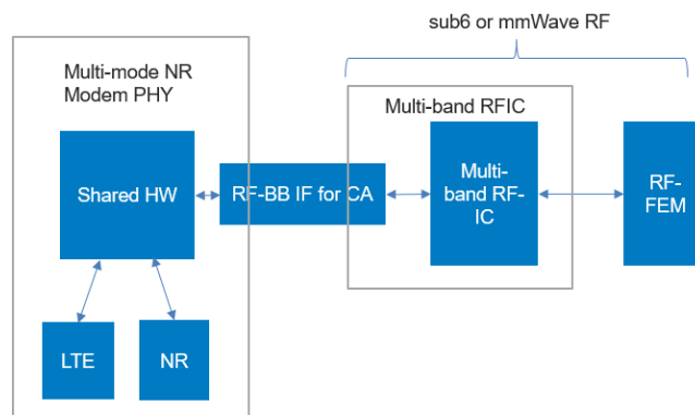
Figure 8-6 Single-chip UE modem architecture for NSA
