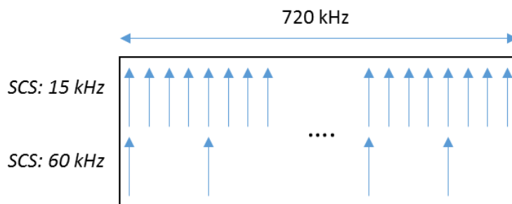
Figure 6-2 Illustration of the subcarrier alignment within one RB of 60kHz numerology
