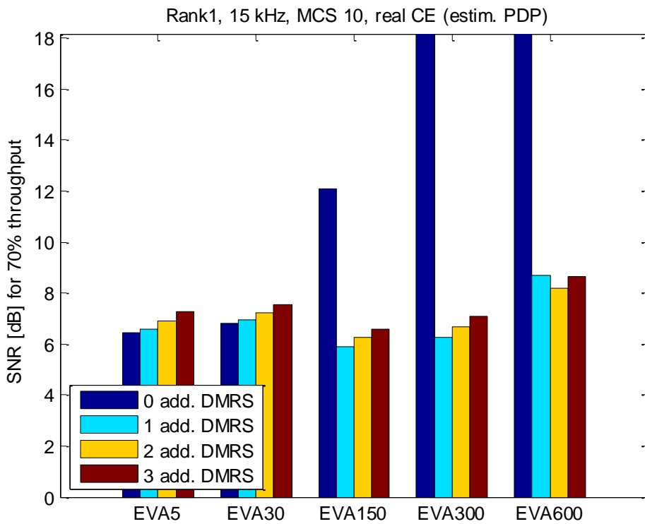
Figure 12-4 An example of NR UE performance with different DMRS configurations under different Doppler spread
