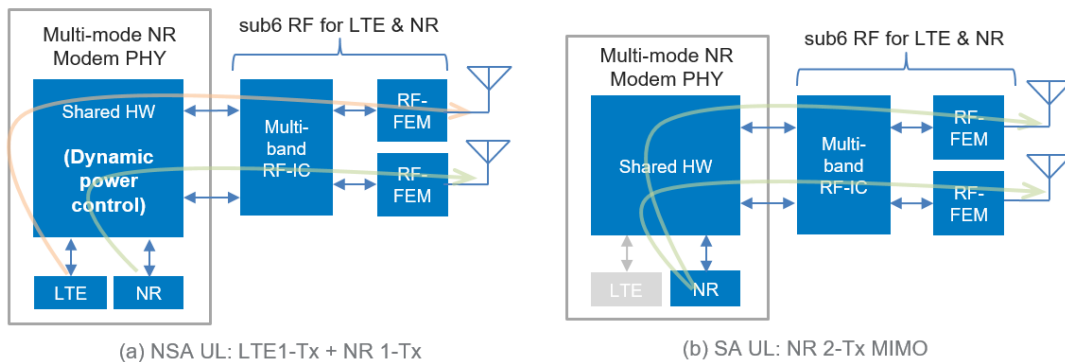
Figure 8-7 LTE+NR Uplink power sharing in NSA and 2-Tx UL-MIMO in SA
