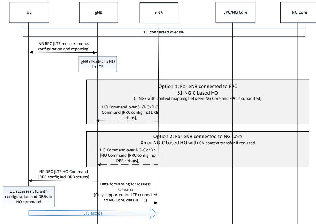
Figure 9-2 NR to LTE Connected state mobility
