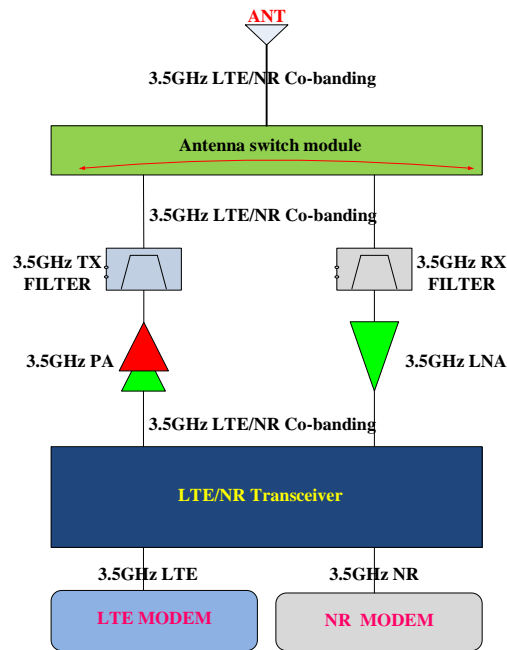
Figure 11-7 3.5GHz typical RF architecture
