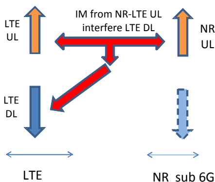
Figure 11-5 Illustration of interference from IMD
