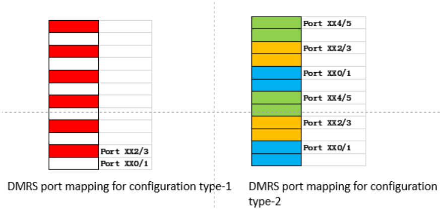
Figure 6-6 Illustration of DMRS port mapping
