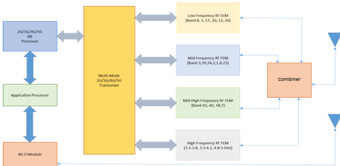
Figure 7-1 MMMB architecture 1
