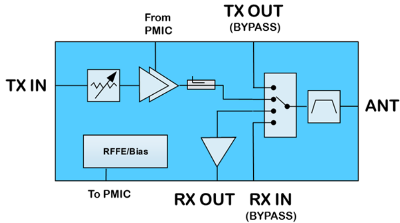
Figure 13-3 RF front end module block diagram
