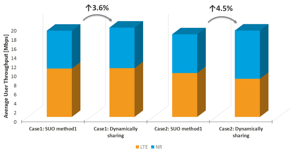
Figure 11-10 SUO vs. DPS, Average User Throughout of all UE
