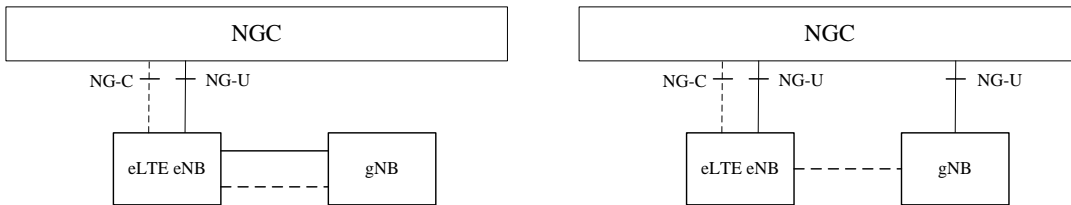
Figure 8-4 Non-Standalone NR – 3GPP Options 7 and 7A
