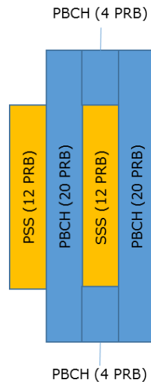
Figure 6-5 Illustration of SS/PBCH block mapping
