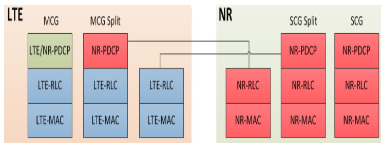
Figure 8-8 NR PDCP aggregation/split for MCG and SCG radio bearer split support in NSA Option3/3x
