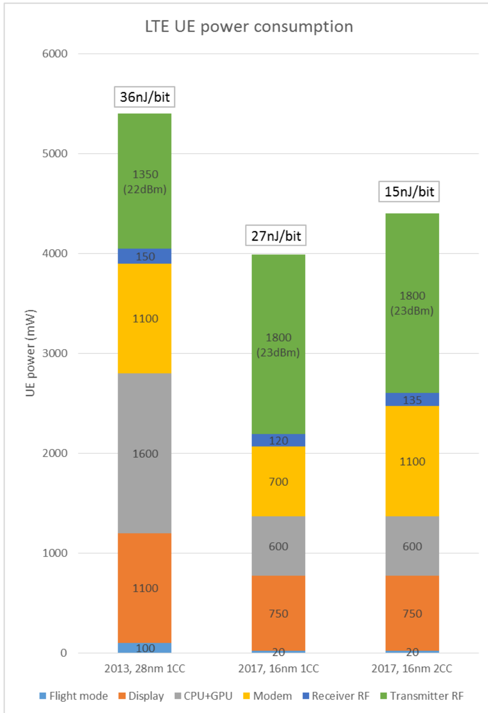
Figure 13-1 LTE UE power consumption
