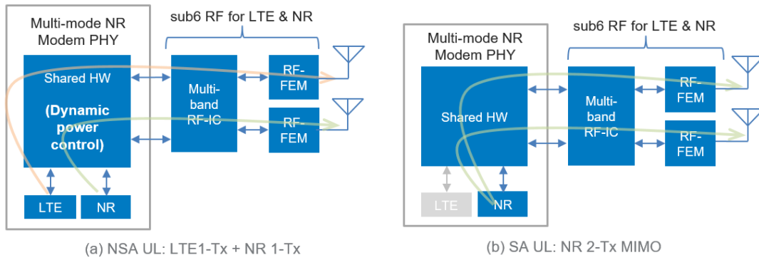
Figure 8-7 LTE+NR Uplink power sharing in NSA and 2-Tx UL-MIMO in SA
