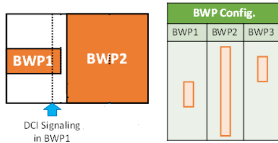
Figure 6-3 Illustration of DCI-based active BWP switching
